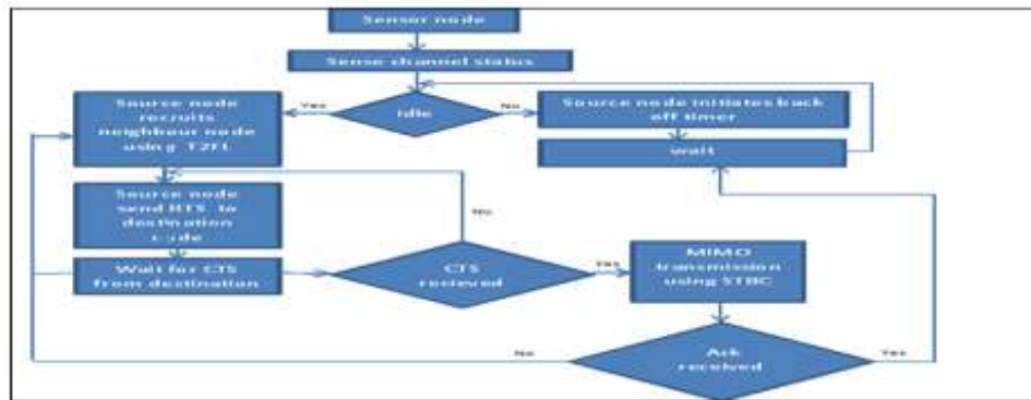
Fig.2.1 Flowchart for cooperative MIMO MAC protocol using T2FL.
